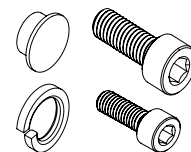
SPARE PARTS 1 x BOLT COVER 1 x M8 25mm BOLT 1 x M8 SPRING WASHER 1 x M5 12mm BOLT
